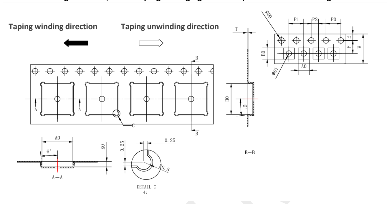
Figure 6-6: QFN7*7 Taping Packaging Carrier Tape Dimension Drawing
