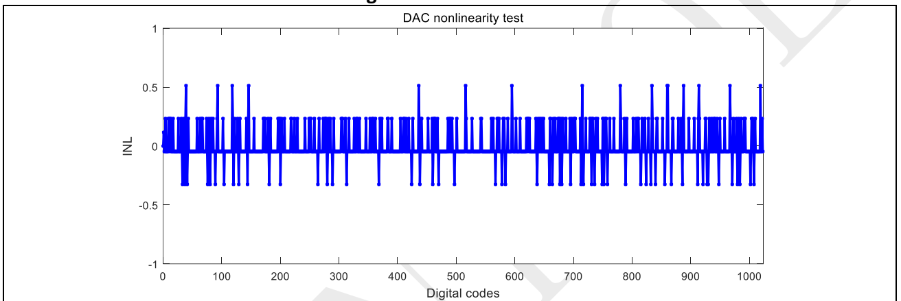
Figure 5-13: INL curve
