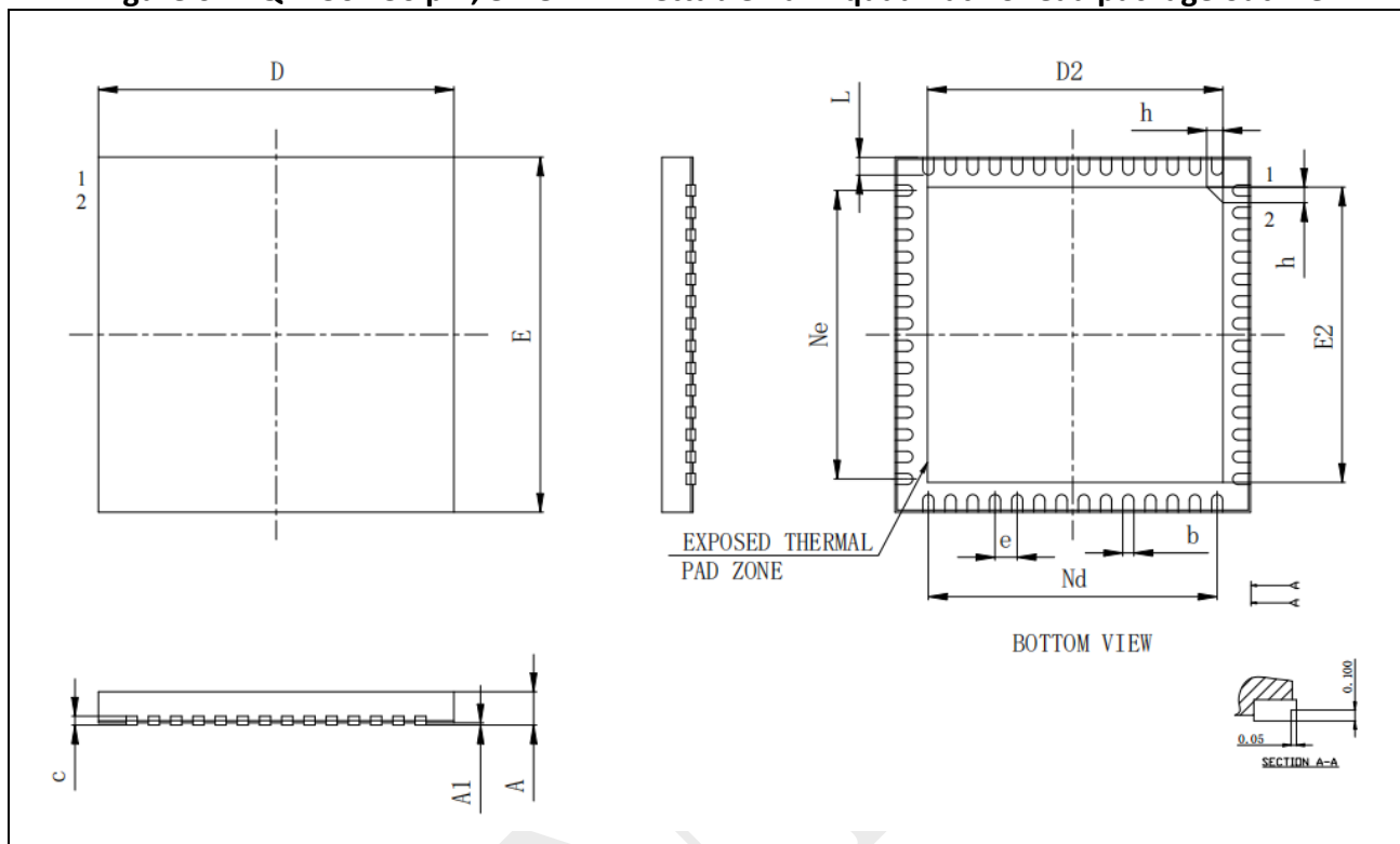
Figure 6-4: QFN56 - 56 pin, 8 x 8 mm wettable flank quad flat no-lead package outline
