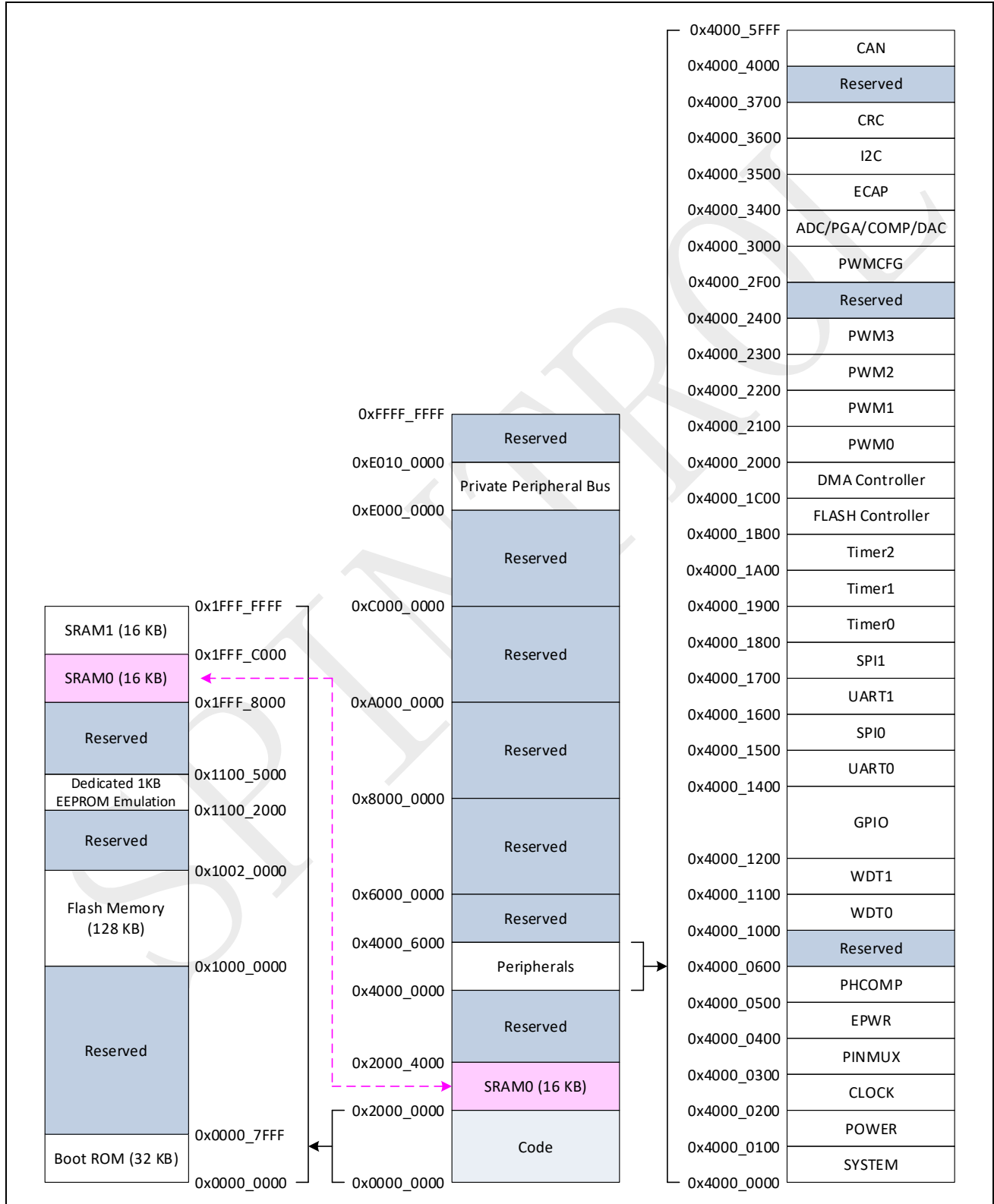
Figure 4-1: Memory map
