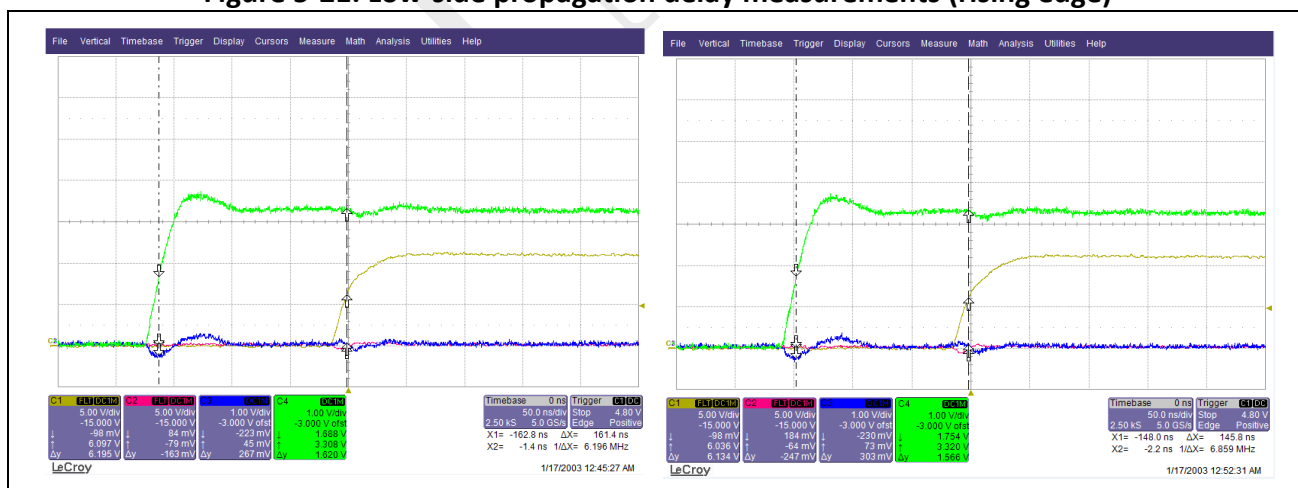
Figure 5-21: Low-side propagation delay measurements (rising edge)
