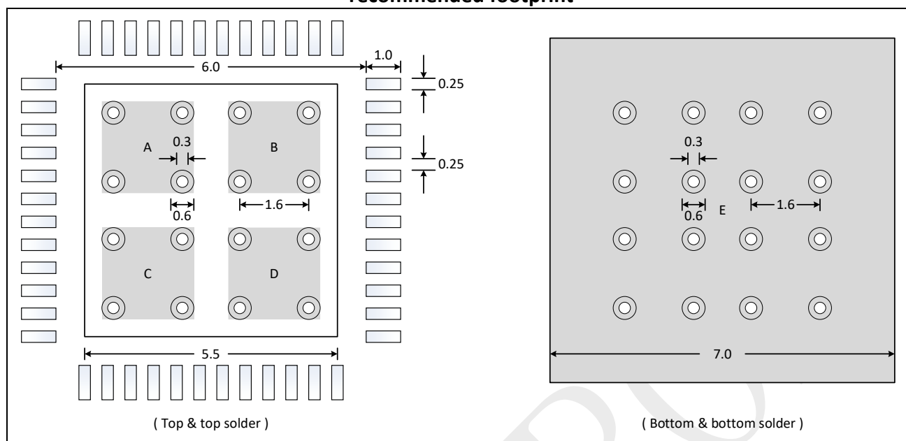
Figure 6-2: QFN48 - 48 pin, 7 x 7 mm wettable flank quad flat no-lead package recommended footprint
