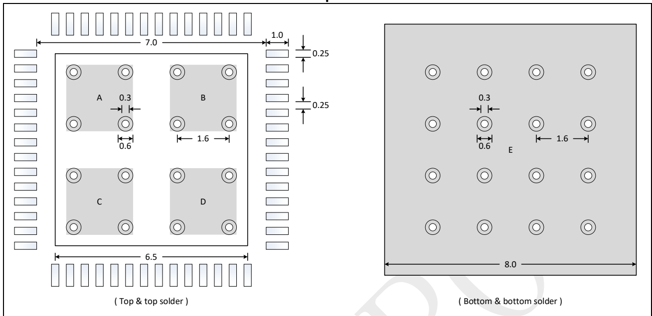
Figure 6-5: QFN56 - 56 pin, 8 x 8 mm wettable flank quad flat no-lead package recommended footprint
