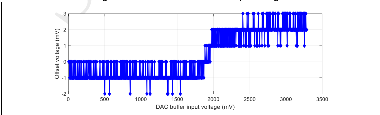
Figure 5-14: DAC buffer offset over Input voltage
