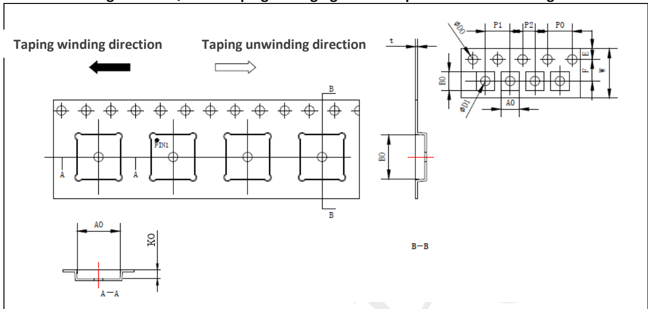
Figure 6-3: QFN7*7 Taping Packaging Carrier Tape Dimension Drawing
